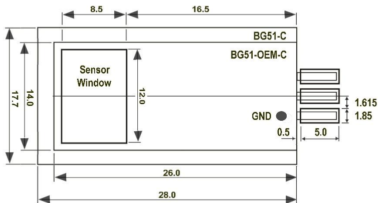
Dimensions in mm Top View
